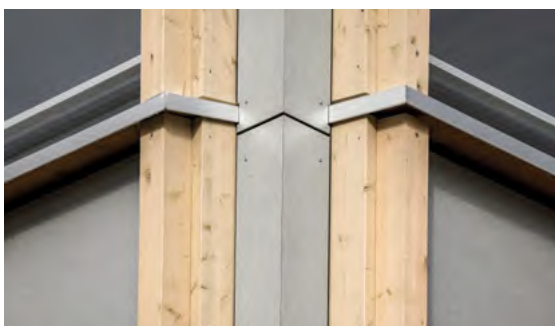
Visible mounting combined with the Closed Corner 90° system
