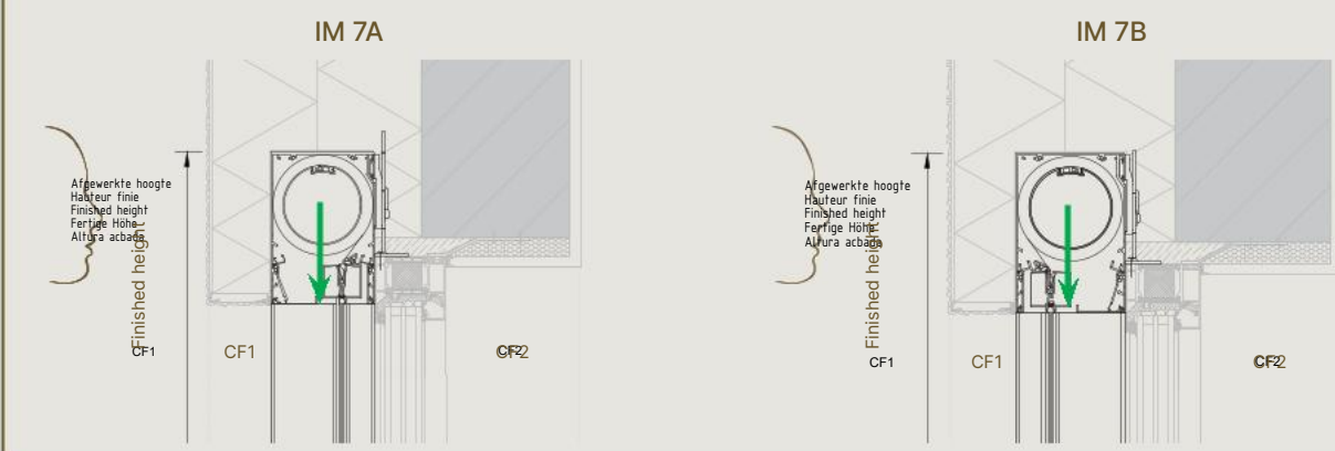
Medium - Drawing recessed plaster - Base box M.W+
