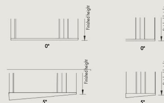
Base plate side guiding channel
