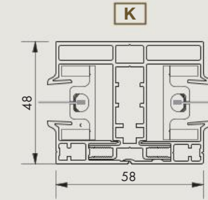
K = coupling side guiding channel*
