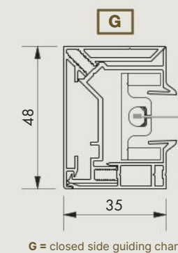
Side guiding channels
