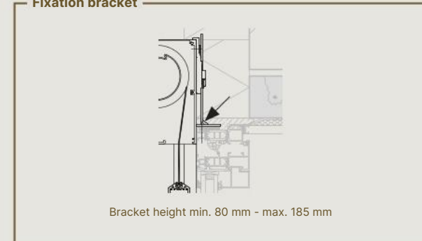
Fixation bracket
