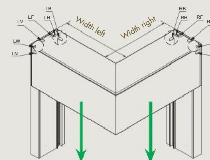
Cable feed
