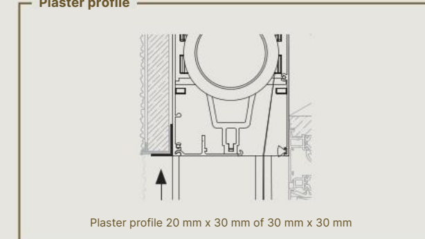
Plaster profile
