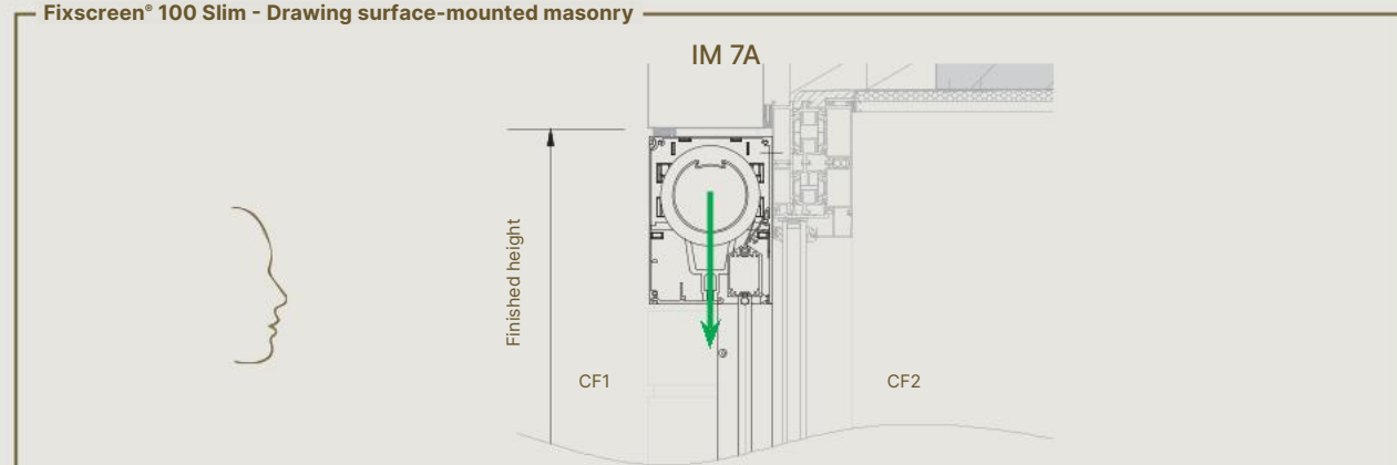
Fixscreen® 100 Slim - Drawing surface-mounted masonry
