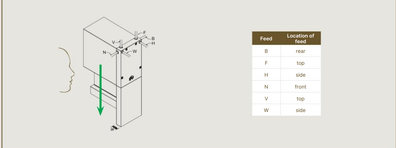
Cable feed
