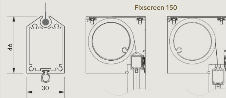
FH ≤ 2800 mm Bottom bar disappears completely in the head box
