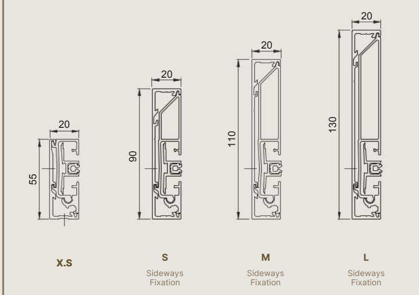
Side guiding channels
