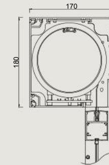
Cross section
