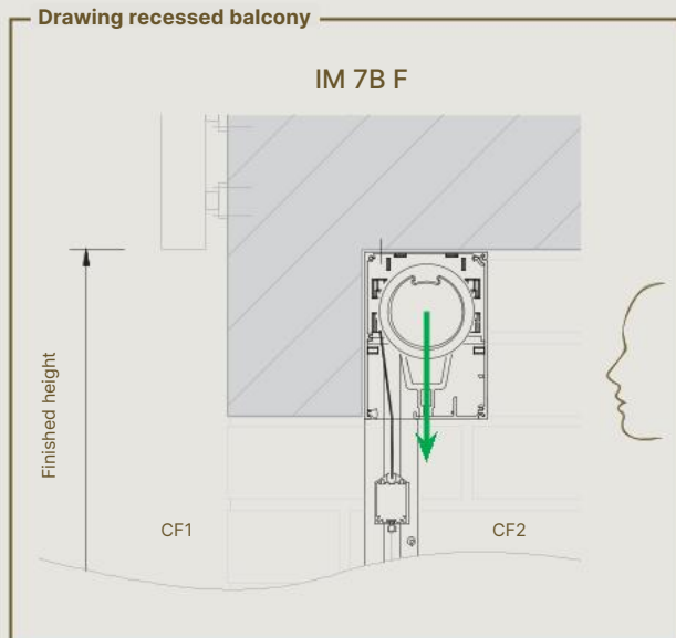
Drawing recessed balcony
