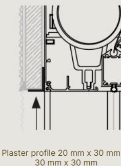
Plaster profile
