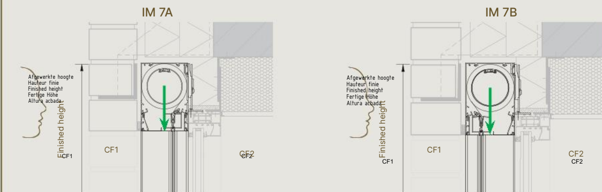
Medium - Drawing recessed masonry
