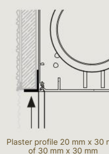
Plaster profile
