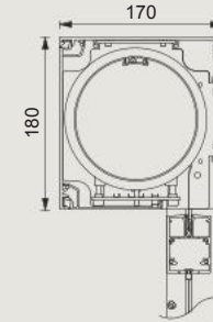
Cross section
