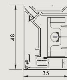
G = closed side guiding channel
