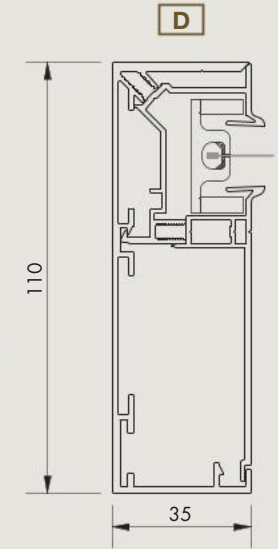
D = deep side guiding channel (standard)
