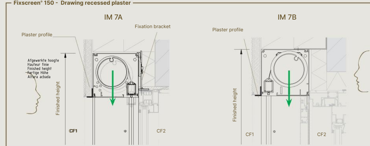
Fixation bracket
