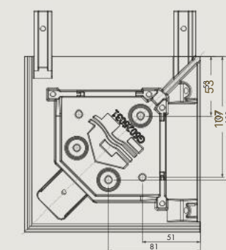
Angle bracket (position of drill holes)
