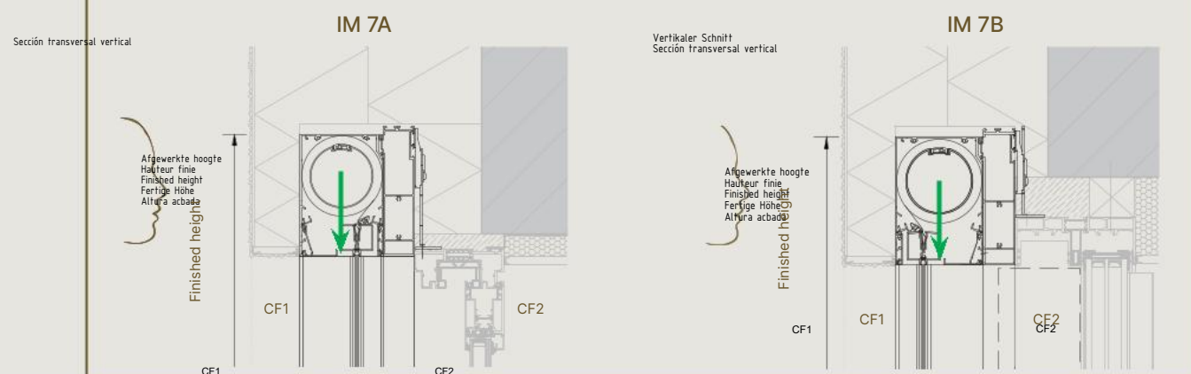
Medium - Drawing recessed plaster - Base box M.W+
