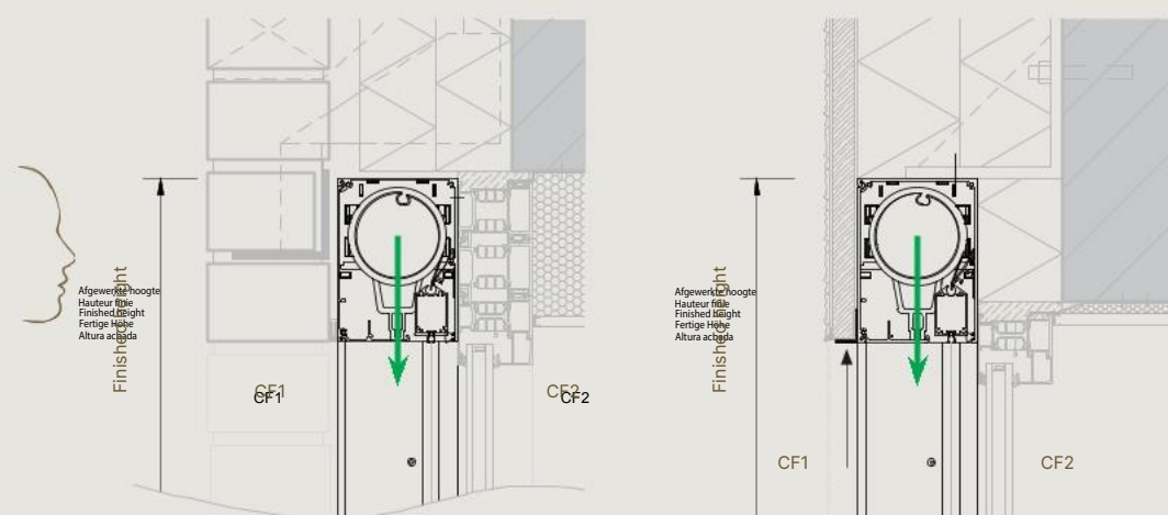
Drawing surface-mounted masonry
