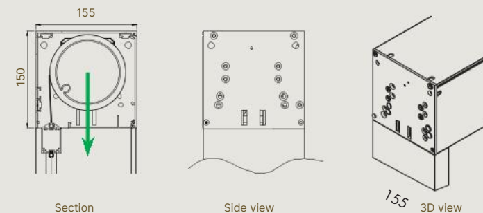
Head box
