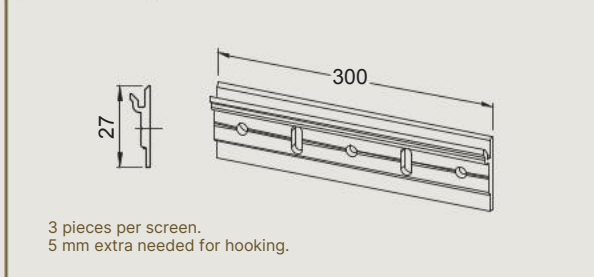
Hook profile
