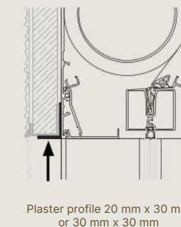
Plaster profile
