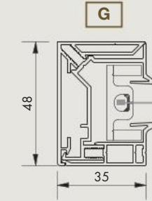
G = closed side guiding channel
