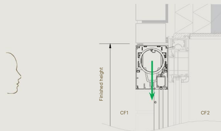
Drawing surface-mounted masonry
