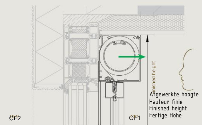
Small - Drawing surface-mounted indoor application
