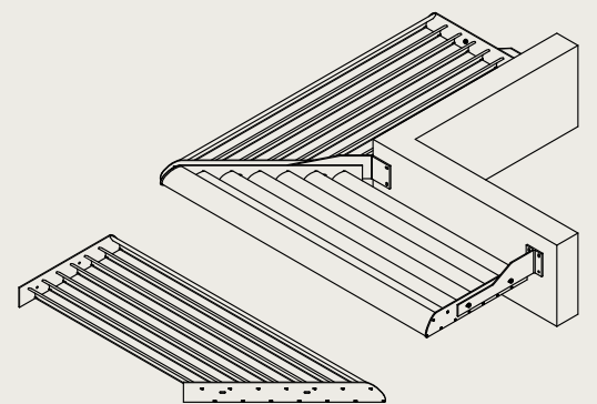
expansion joint on the corner
