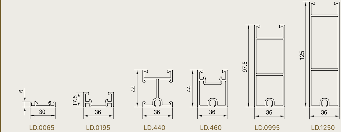
End caps for mullions
