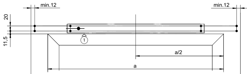
Side limit (e.g. post or jamb) | 1 = Top edge leaf
