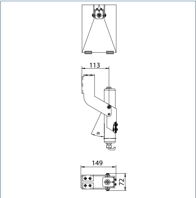
INWARD opening console
