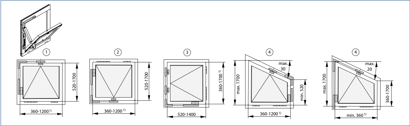
All dimensions in mm 1 = Bottom-hung window | 2 = Top-hung window | 3 = Side-hung window | 4 = Pitched window tilt | 1) For PVC windows Solo max. 800 mm
