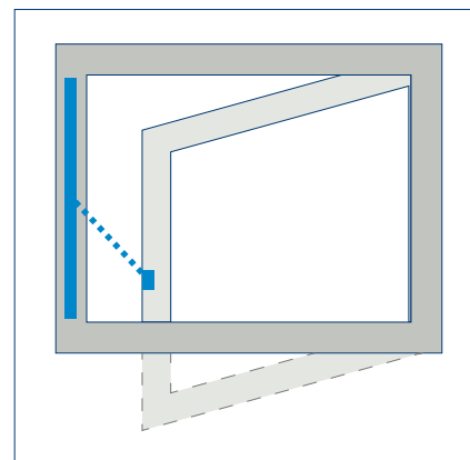
Side-hung leaf DIN L OUTWARD opening (drive cannot be swivelled)
