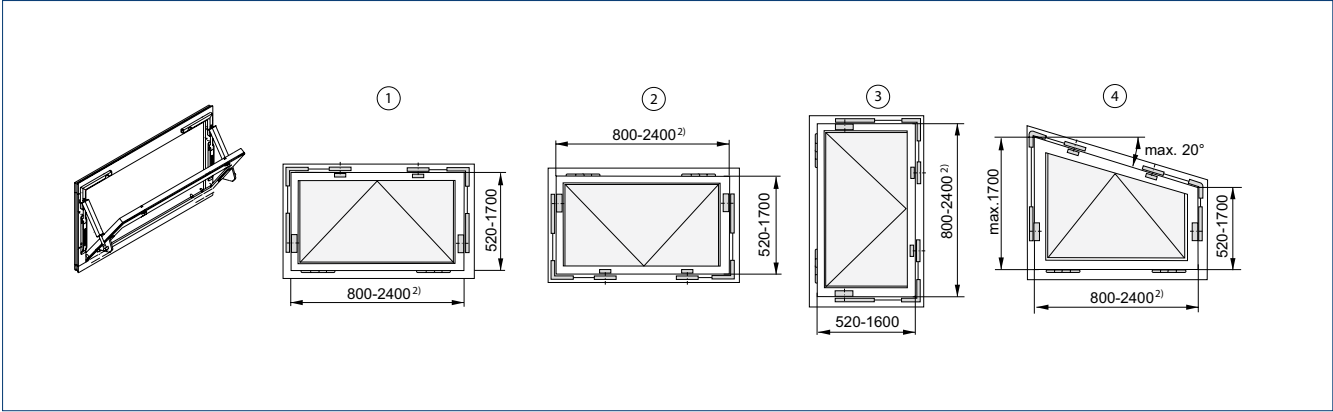
All dimensions in mm 1 = Bottom-hung window | 2 = Top-hung window | 3 = Side-hung window | 4 = Pitched window | 2) For PVC windows Syncro max. 1600 mm
