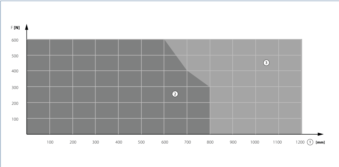
F = Force | 1 = Stroke | 2 = Pressure | 3 = Tension
