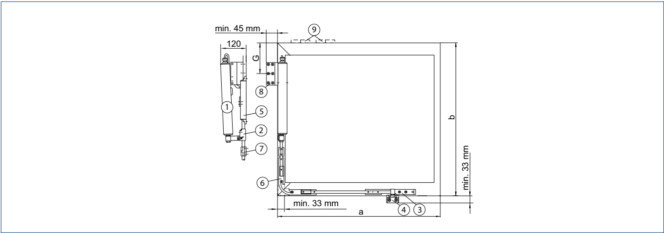
For details of fitting dimensions G and E, see table a = Leaf width | b = Leaf height | 1 = Electric spindle drive E 350 | 2 = Rod transmission | 3 = Additional locking OL 320 | 4 = Additional bracket complete | 5 = Release spring | 6 = Corner transmission OL 320 | 7 = Rod guide OL 320 | 8 = Frame angle | 9 = 2 hinges on the drive side (to be provided by the customer)
