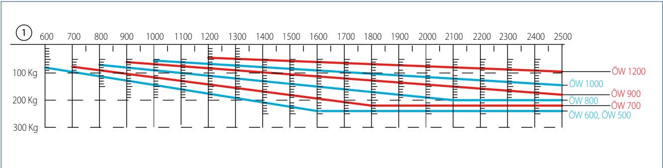
LEAF WEIGHT (MAX.) IN KG FOR DIMENSION X DETERMINED AND GIVEN-OPENING WIDTH FOR 2 SAFETY SCISSORS NO. 60 PER WINDOW
