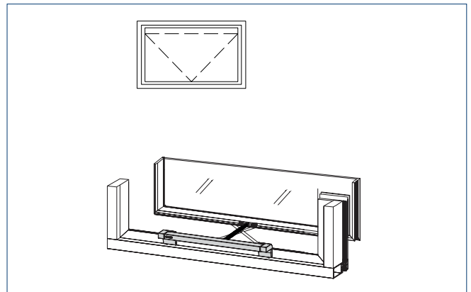
Frame installation OUTWARD opening projected top-hung window
