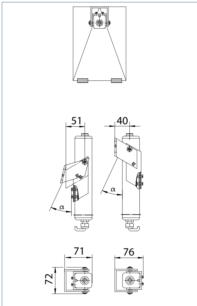
Standard bracket
