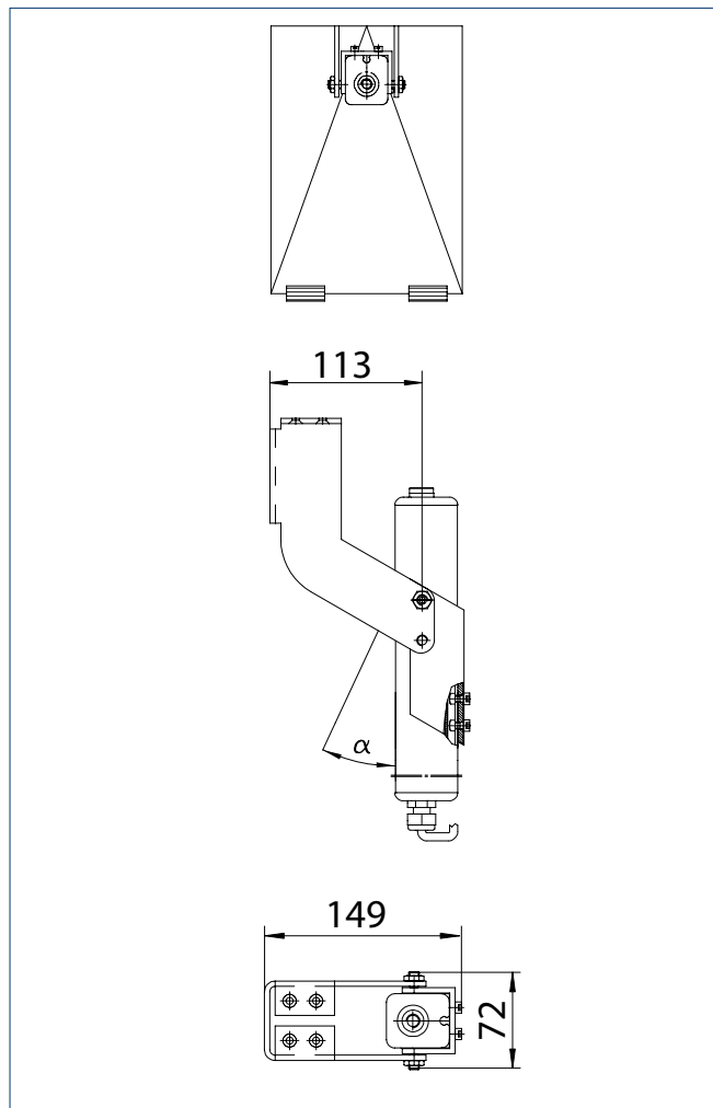
INWARD opening bracket
