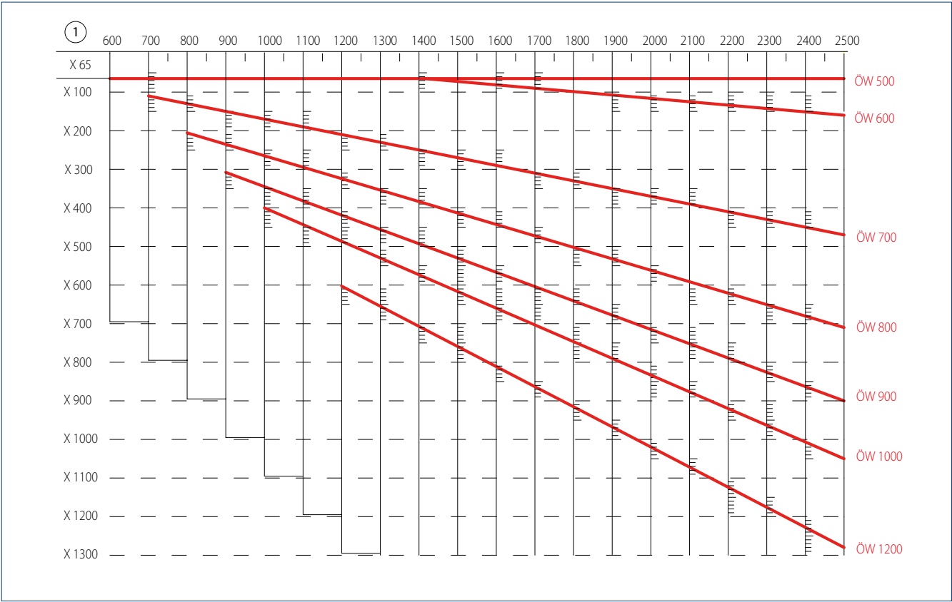
DETERMINATION OF INSTALLATION DIMENSION X FOR SAFETY SCISSORS NO. 60 FOR-OPENING WIDTHS 500, 600, 700, 800, 900, 1000 AND 1200 MM
