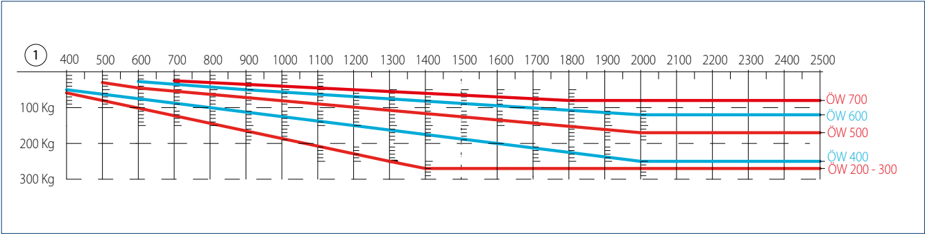
LEAF WEIGHT (MAX.) IN KG FOR DETERMINED DIMENSION X AND SPECIFIED OPENING WIDTH FOR 2 SAFETY SCISSORS NO. 35 PER WINDOW
