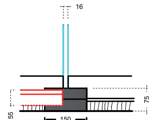
DETAIL D
