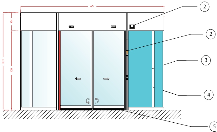
FRONTAL VIEW
