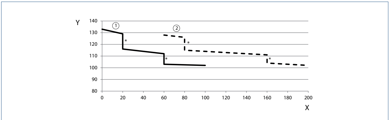
* = Preload | X = Reveal depth (mm) | Y = Max. door opening angle (°) | 1 = Lever 330 mm | 2 = Lever 450 mm
