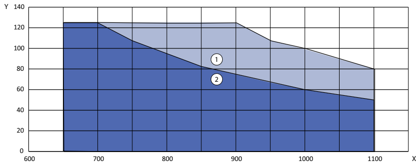
X = Door width (mm) | Y = Door weight (kg) | 1 = Area of application in low-energy mode | 2 = Area of application in automatic mode
