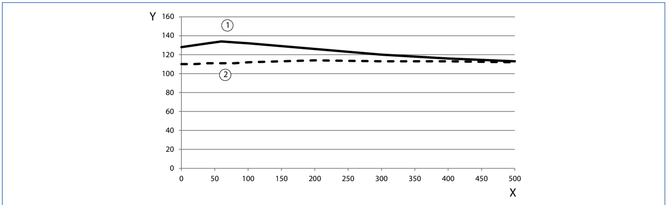
X = Reveal depth (mm) | Y = Max. door opening angle (°) | 1 = Door opening angle | 2 = Door opening angle with sensor link arm
