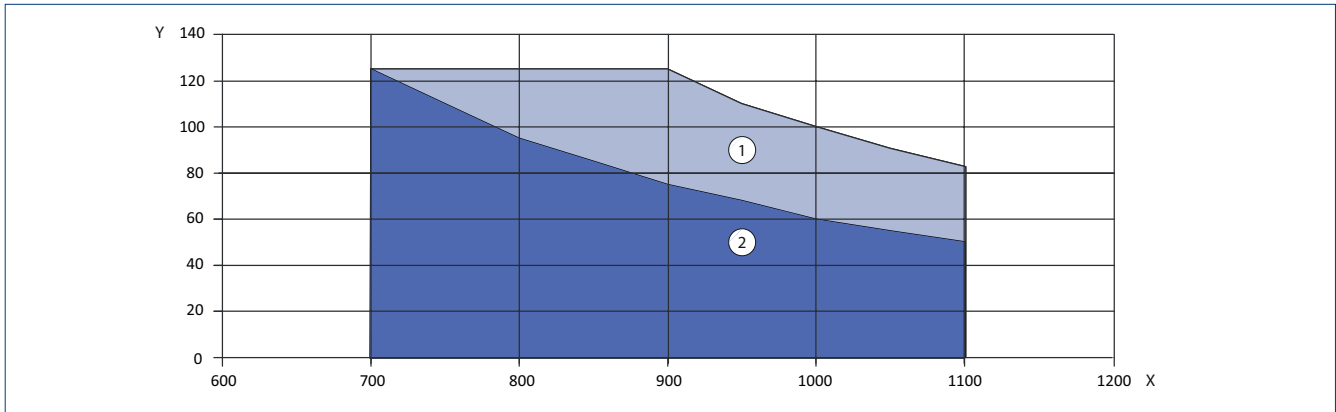
X = Door width (mm) | Y = Door weight (kg) | Minimum door width for installation in metal door or frame 750 mm
